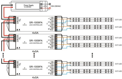
2) Receiver Connection Diagram for Multiple Units
